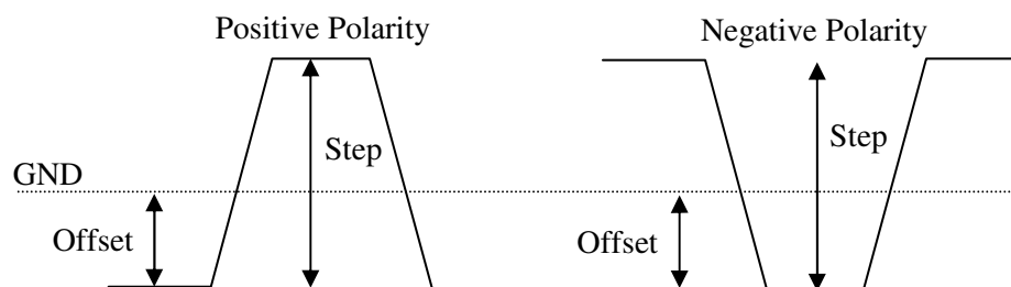
Figure 12: Output Level Configuration
