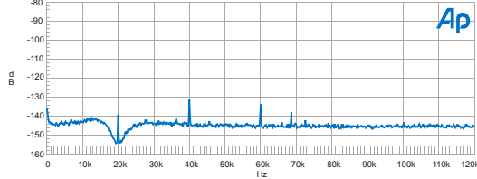
Figure 4. Typical residual THD+N spectrum at 20 kHz, 2 Vrms. (32768 point FFT of notch filter output, Sample Rate = 262 ks/s, 16 averages).
