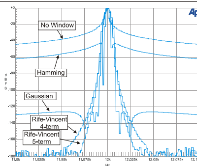
Figure 26. Windowing functions for FFT (A) Figure 27. Windowing functions for FFT (B)
