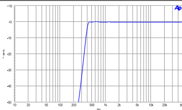
Figure 20. FHP-400. 400 Hz 9-pole High Pass Filter.
