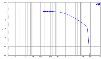
Figure 16. FIL-D75F. 75 \mu\text{s} with 19 kHz (FM) notch De-emphasis Filter.
