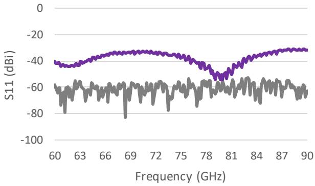
Typical Reflection Loss
