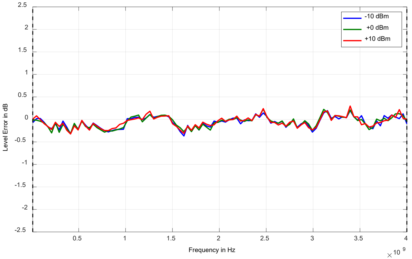
Figure 4: Level accuracy
