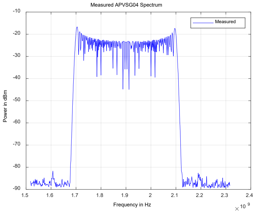
Figure 7: Wideband FM (1MHz rate, 200 MHz deviation)
