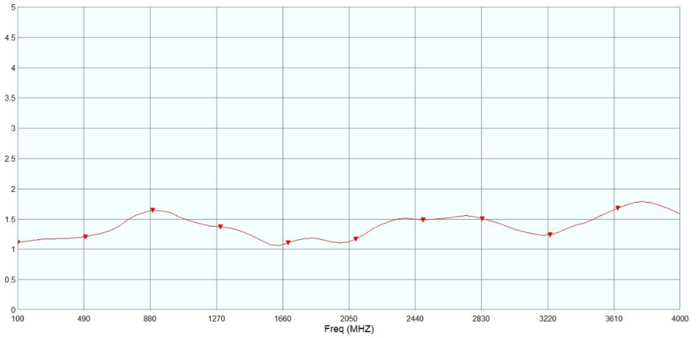
Figure 18: Typical VSWR (APVSG12)
