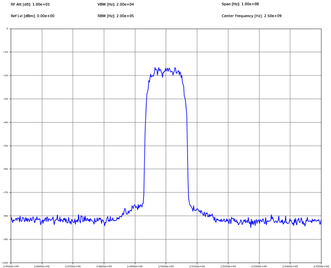
Figure 12: 256QAM 10 MS/s
